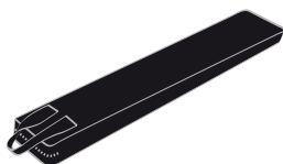
Art nr.: 2.11.07103-01 Weight: 0,24 kg Material: nylon Dimensions: 150 x 50 x 730 mm
