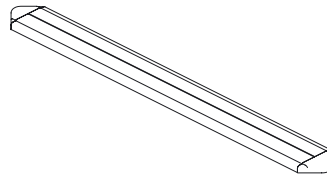
Art nr.: 2.46.01001 Weight: 0,12 kg Material: aluminium alloy, eloxed magnetic tape
